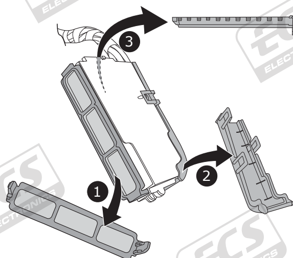
Fusebox 5 RD
